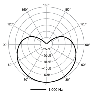
Polar Pattern
