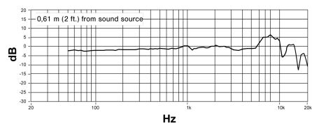
Frequency Response
