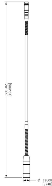
MXC420DF/C Gooseneck Microphone
